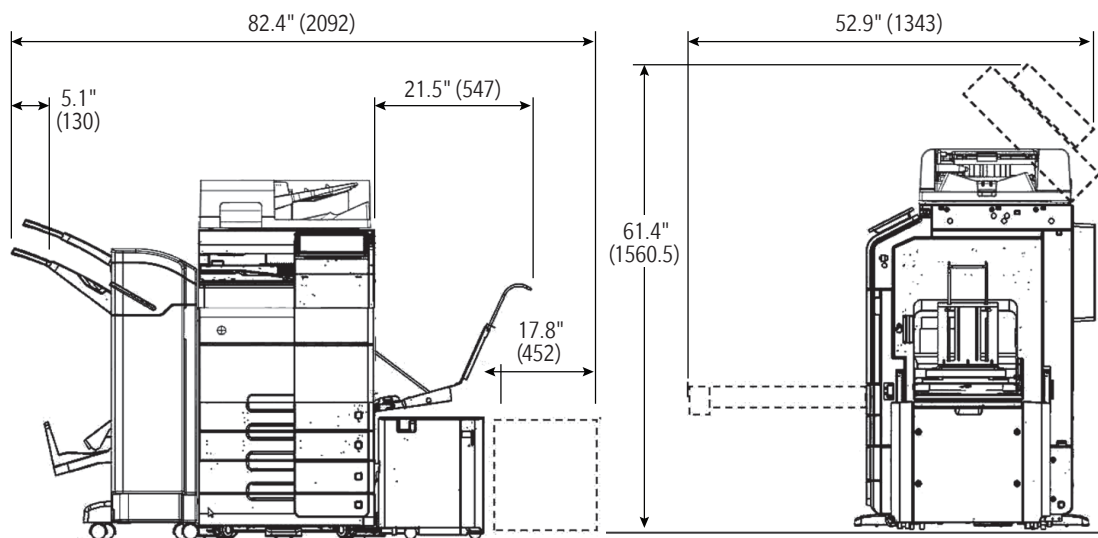
bizhub 650i/550i/450i + FS-539 + LU-302
