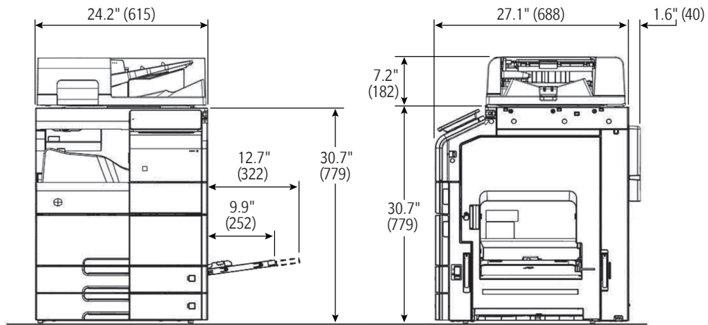
bizhub 650i/550i/450i
