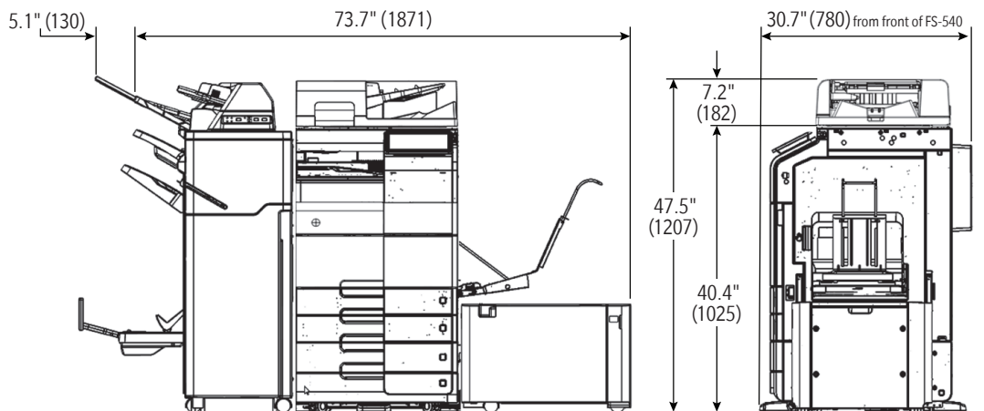
bizhub 650i/550i/450i + LU-207 + FS-540
